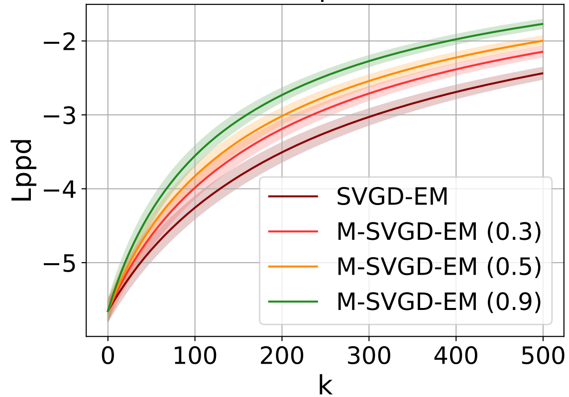
N = 20 particles
