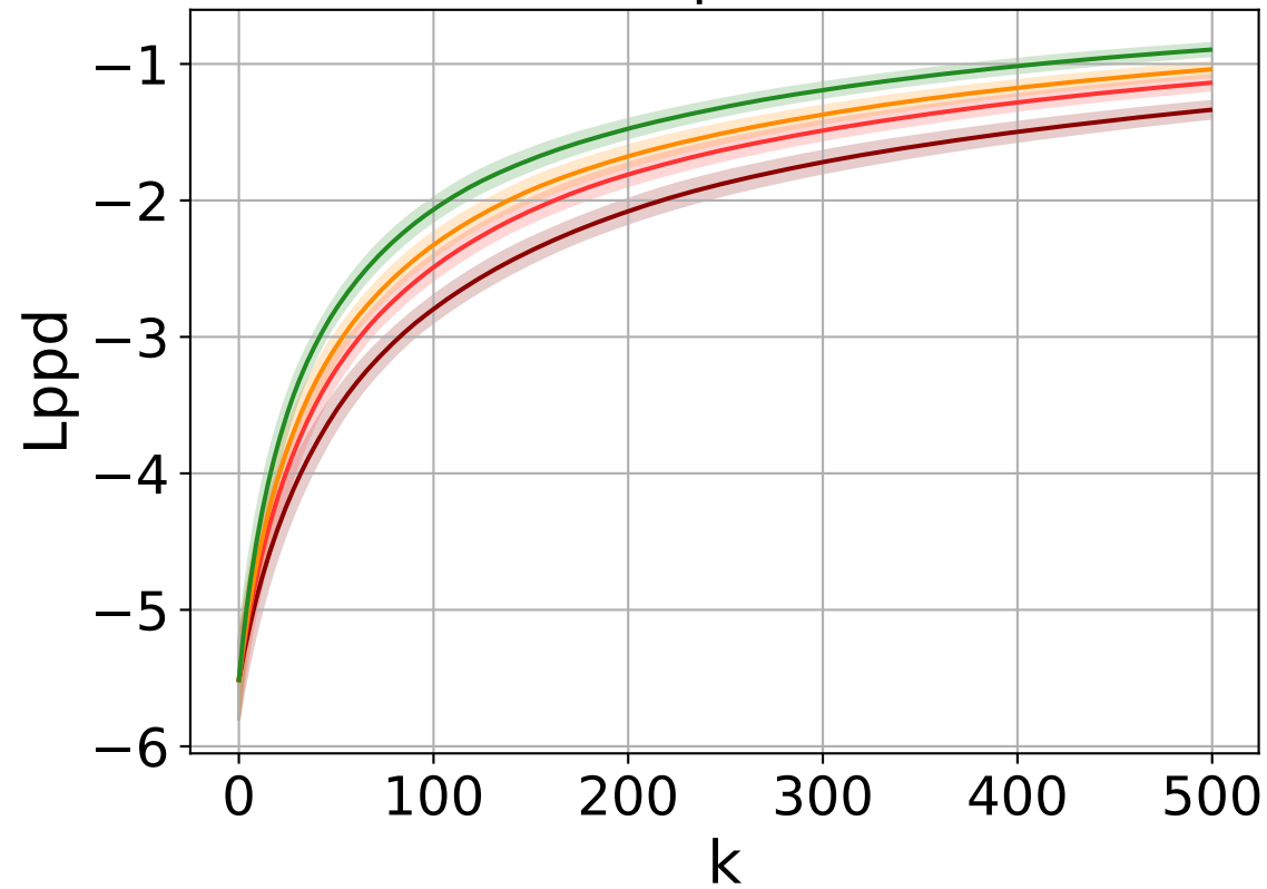
N = 5 particles
