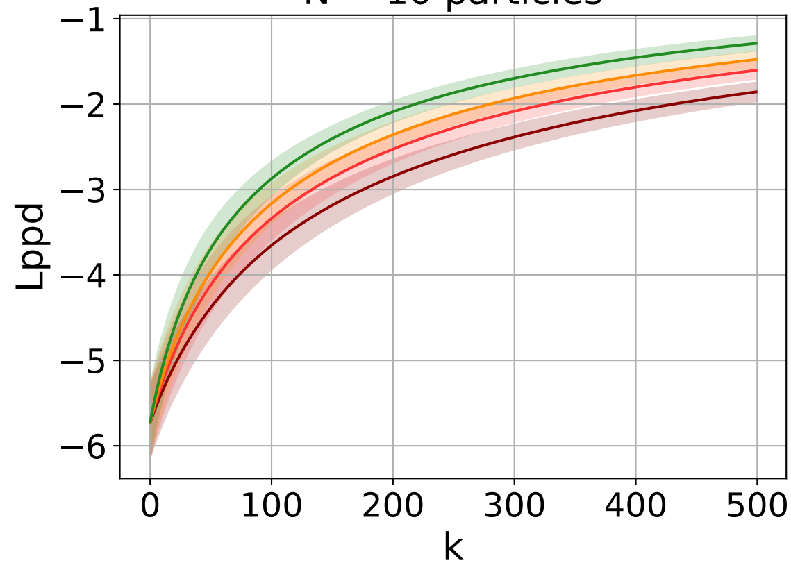
N = 10 particles
